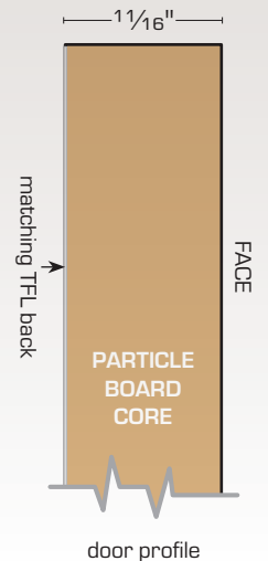
detail of edgebanding (JADE GREEN)
