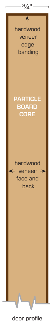
Veneer edgebanding detail (WALNUT)
