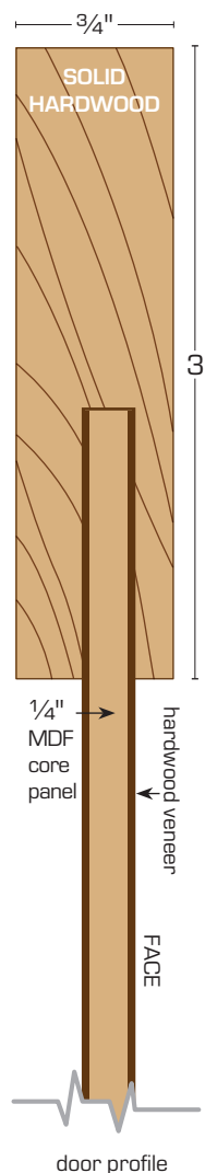
detail of stick-and-cope door frame construction (OAK)
