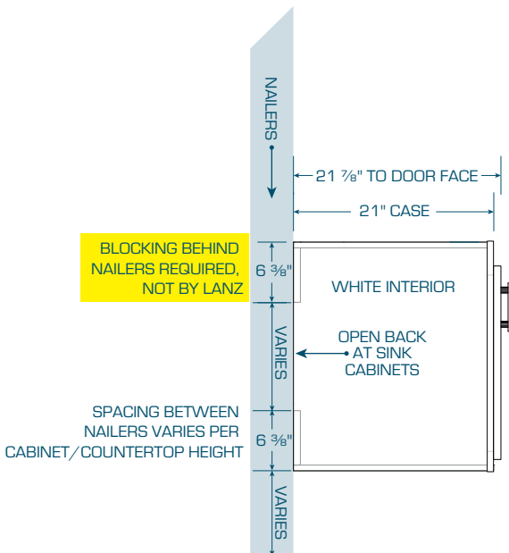
CROSS-SECTION VIEW
