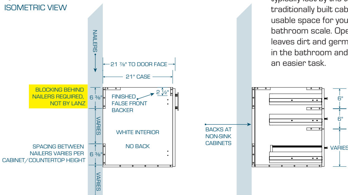
CROSS-SECTION VIEW
